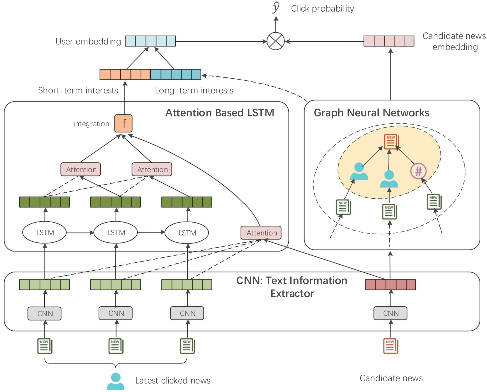
Fig. 1. The framework of GNewsRec.
