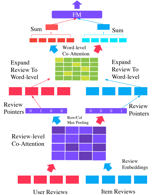
Figure 1: Illustration of proposed model architecture for Pointer-based Learning ( Best viewed in color ). This example illustrates a one pointer example. Review gating mechanism and multi-pointer learning is omitted for clarity.
